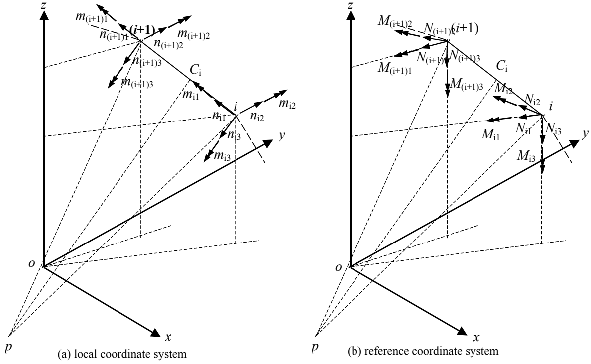
Fig. 10 Components of end force for element
