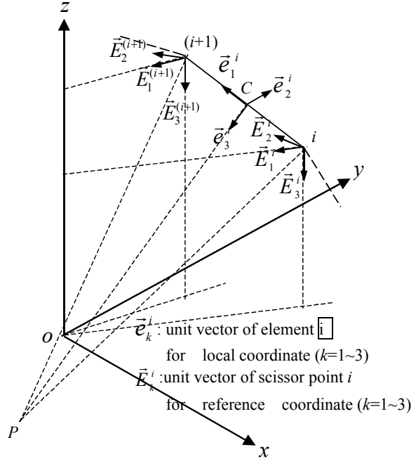
Fig. 9 Base unit orthogonal vectors
