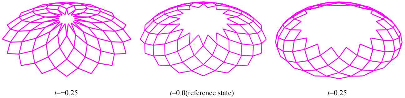
Fig.2 Changing geometry of main structure ( n=6 )
