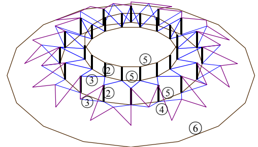
② post ③ diagonal cable ④ zigzag cable ⑤ hoop cable ⑥ outer cable ( : member's changing in length )
