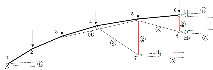
Fig. 7 Diagram of new structural system
