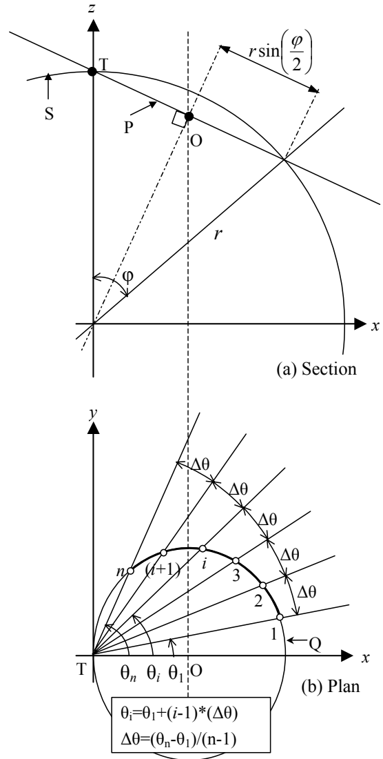
Fig.1 Position of scissor points
